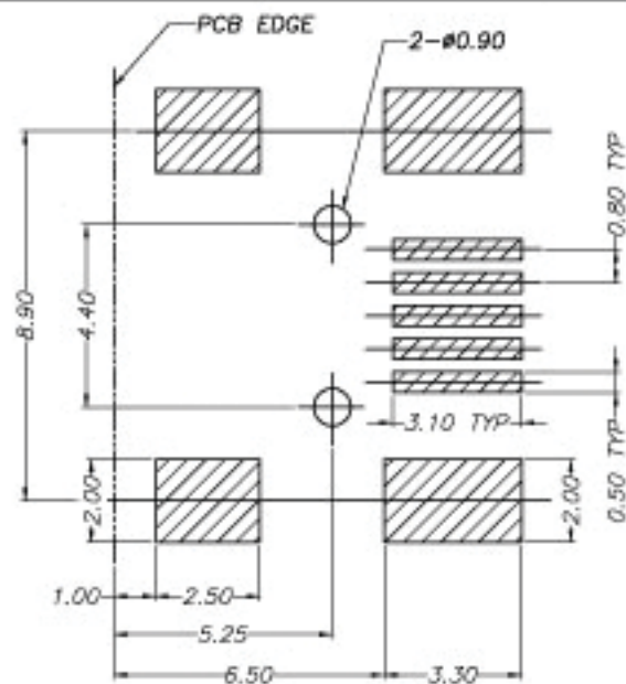
RECOMMENDED PCB LAYOUT (PCB t=0.8)
