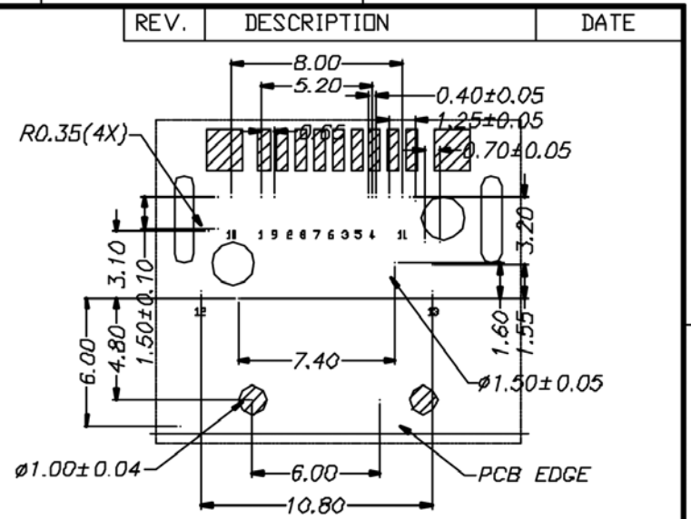
Beta socket PCB footprint SCALE 3:1
