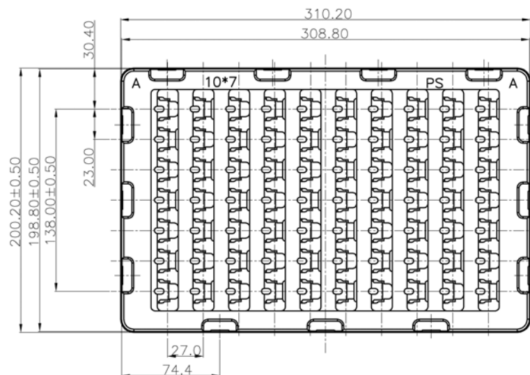
TRAY A LAYOUT
