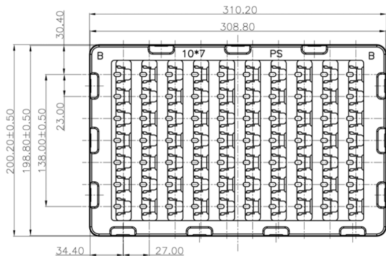
TRAY B LAYOUT
